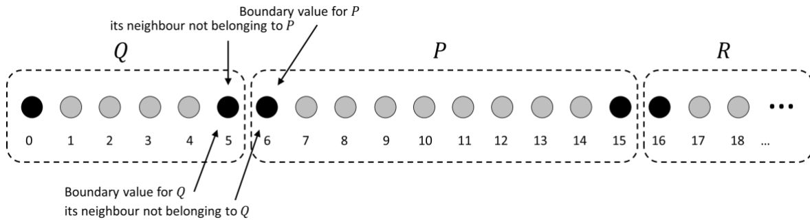
Figure 2: 2-value BVA coverage items for the login example
