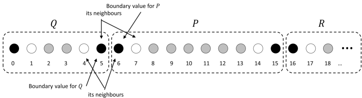
Figure 3: 3-value BVA coverage items for the login example
